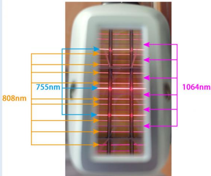
Internal view of handle
